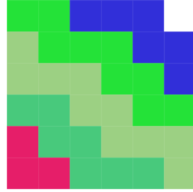
Fig. 6. Here #maximize statements were used with equal priority for all the partitions and 30 models were evaluated, while the sizes are better than in Figure 5, the shapes of the partitions might seem artificial.
