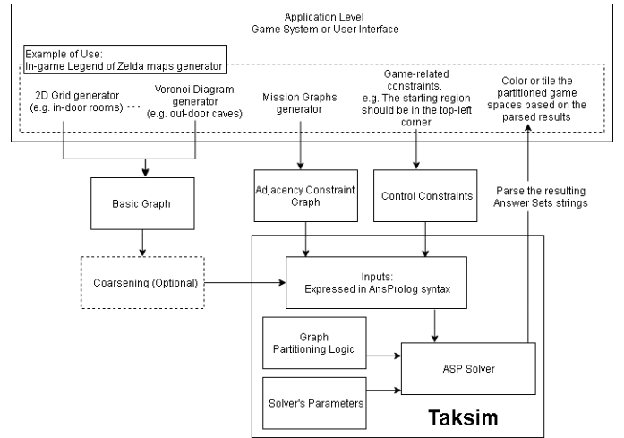
Fig. 3. A system view of Taksim.
