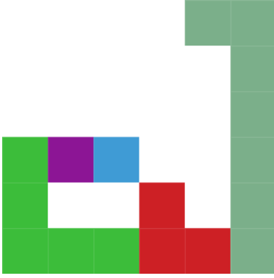
Fig. 5. ASP solver default sample solution. The Constraint Graph is a chain of 5 nodes. White cells are removed nodes.
