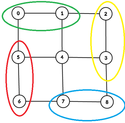
Fig. 2. Reproduced from [3]: We cannot assign the node in the center to any partition
